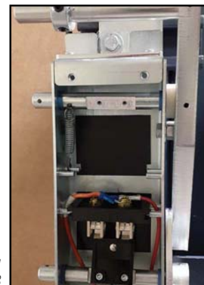
Single Contact PFlintlock Interlock Figure 17-22
