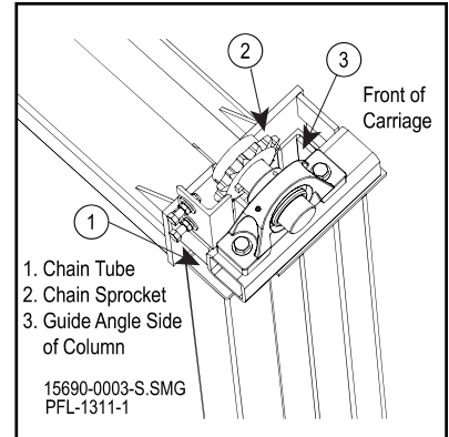
Lower the Tensioner Chain down the Chain Tube Figure 12-43
