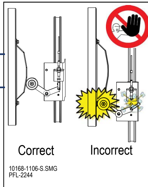
Roller Position Figure 17-16
