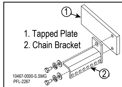
Chain Bracket Figure 12-47
