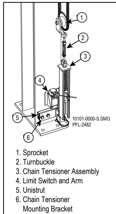
Chain Tensioner Assembly Figure 12-49
