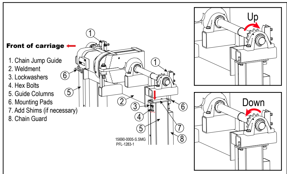
Drivebase Assembly Figure 12-36
