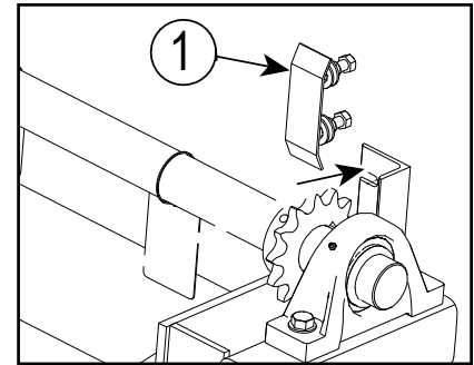
Reinstall the Chain Jump Guides Figure 12-52
