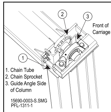
Lower the Tensioner Chain down the Chain Tube Figure 12-43
