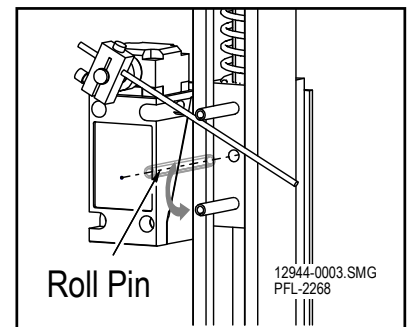
Limit Switch Adjustment Figure 12-51
