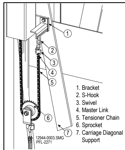
Tensioner Chain Assembly Figure 12-48
