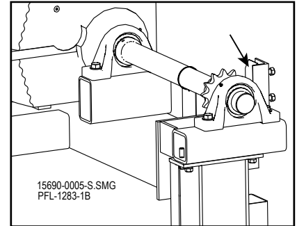
Remove Chain Jump Guide Figure 12-40
