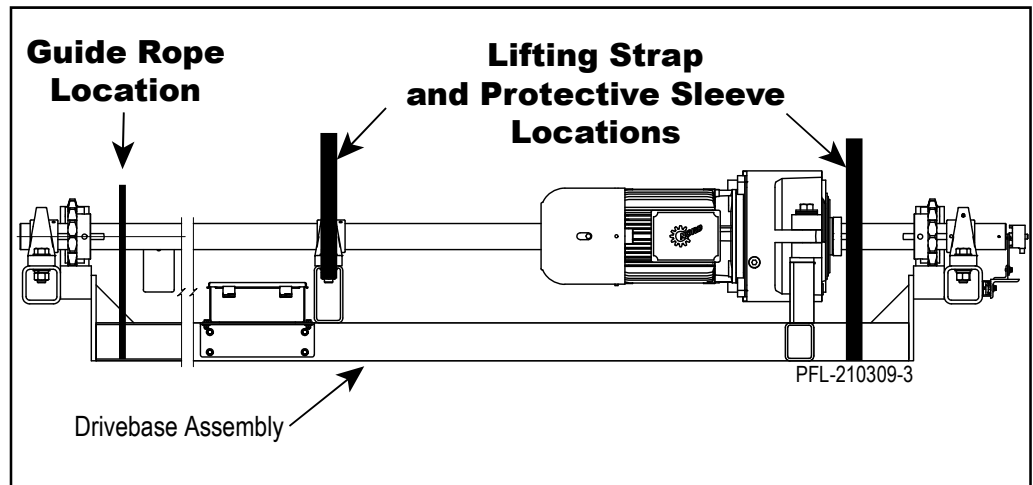
Lifting Drivebase Figure 12-35
