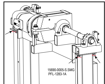
Tighten and Torque Hex Bolts Figure 12-39
