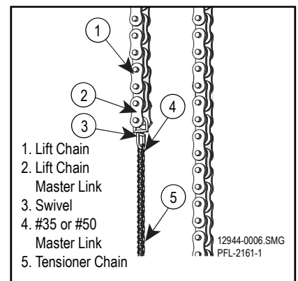
Attach the Tensioner Chain to the Lift Chain Figure 12-42
