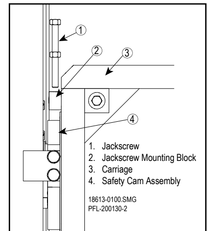
Level with Jackscrew Figure 12-46
