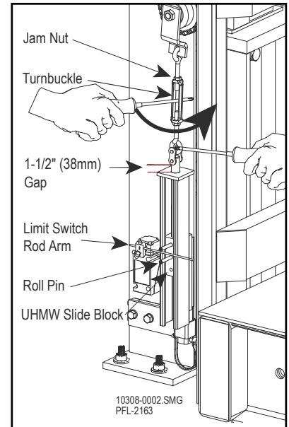
Turnbuckle Adjustment Figure 12-50
