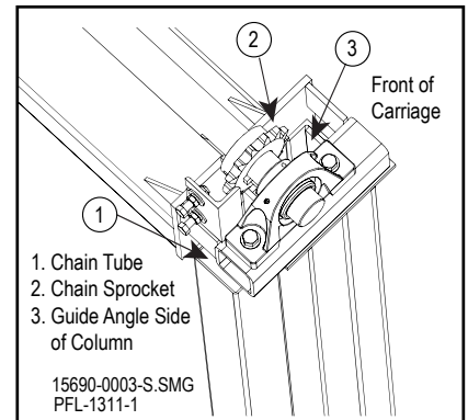
Place a Section over the Chain Sprocket Figure 12-41
