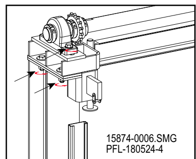
Tighten Hex Head Bolts Figure 12-38
