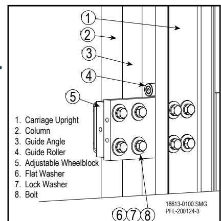
Attach Adjustable Wheelblock Figure 12-19
