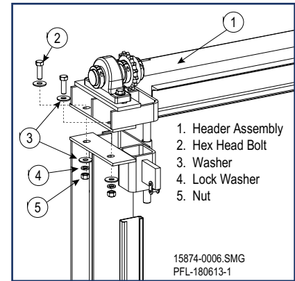
Header Assembly Figure 12-34
