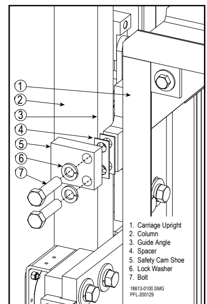
Attach Safety Cam Shoe Figure 12-30
