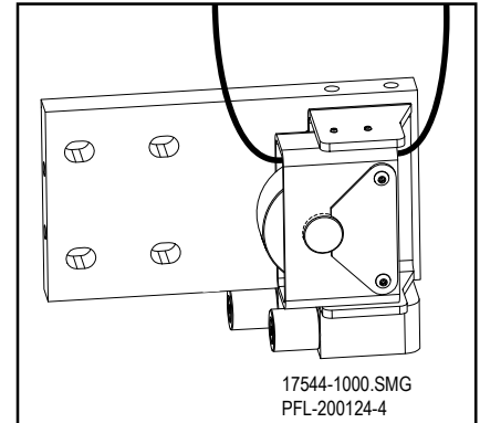
Upper Wheelblock Orientation Figure 12-20
