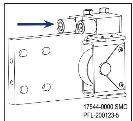
Attach Guide Roller Block Assembly Figure 12-16
