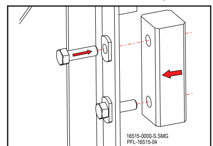
Attach Guide Blocks Figure 16-55
