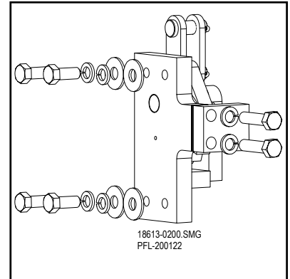
Remove Hex Head Screws Figure 12-24
