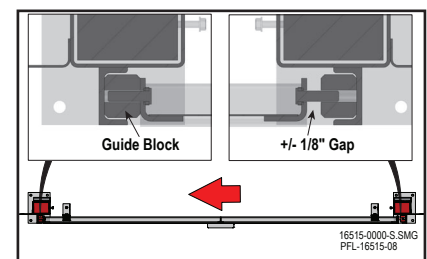
Guide Block Gap Figure 16-91
