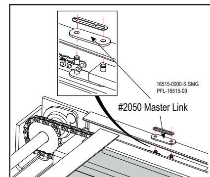
Connect Master Link Figure 16-43
