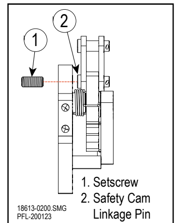
Insert Setscrew Figure 12-27
