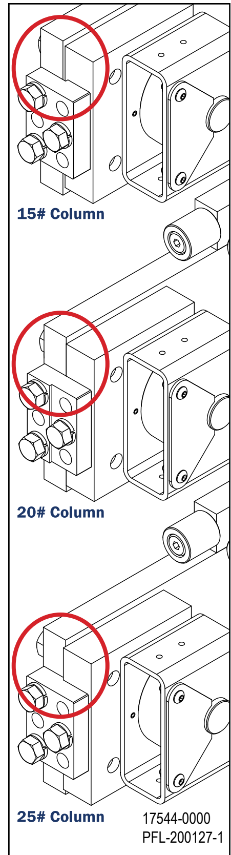
Clamp Bar Positions Figure 12-23
