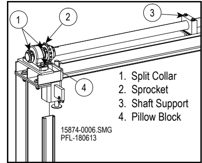
Tighten Setscrews and Shaft Support Bolts Figure 12-42
