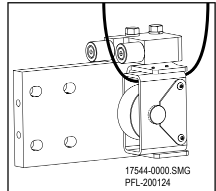
Lower Wheelblock Orientation Figure 12-17
