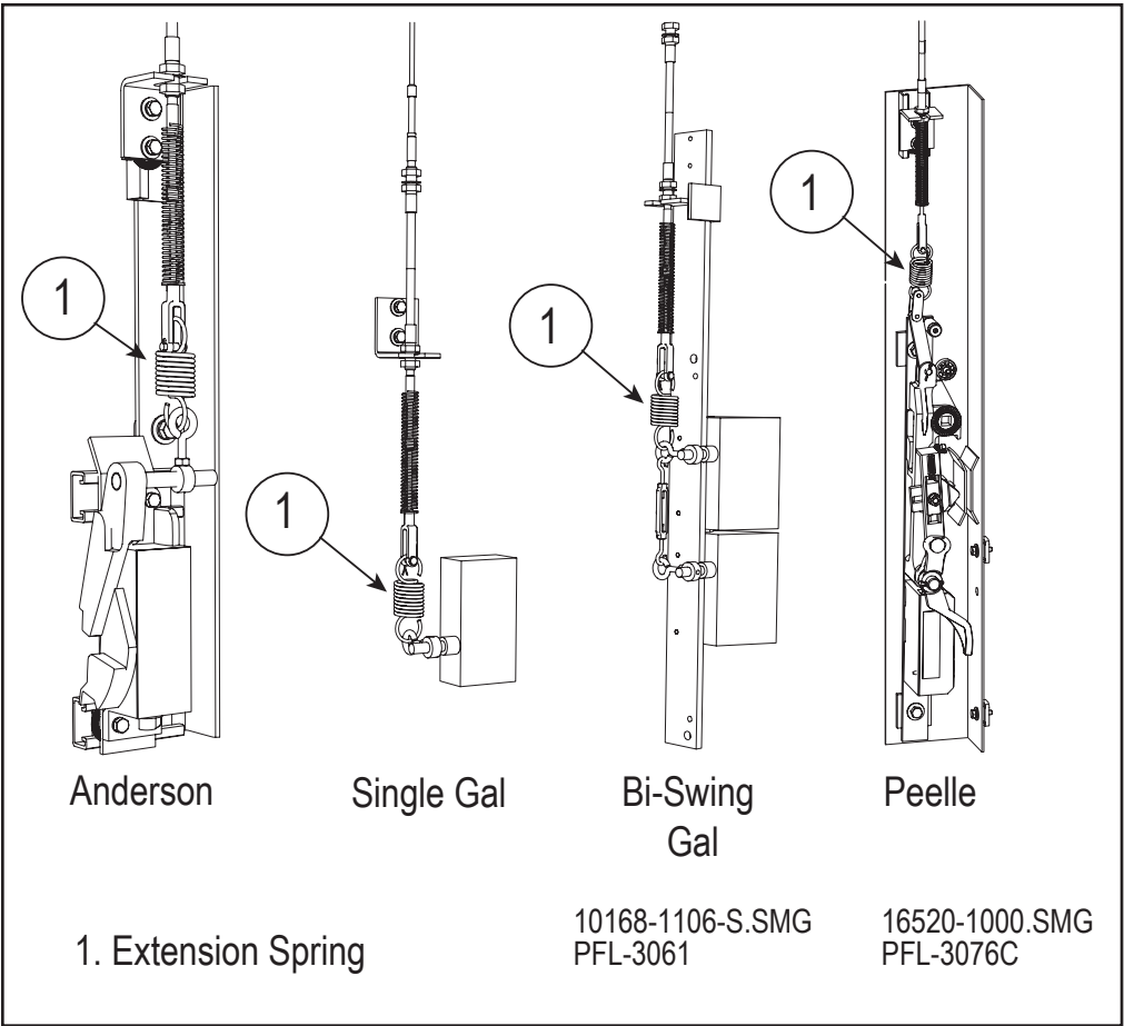
Cable Interlocks Figure 17-1
