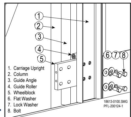
Lower Wheelblock Placement Figure 12-18
