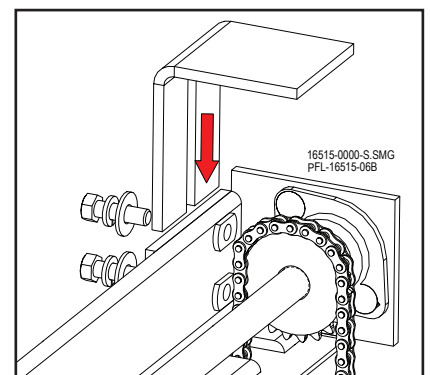
Position Chain Jump Guides Figure 16-52
