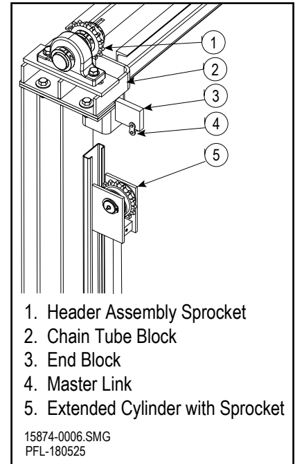
Extend the Hydraulic Cylinder Figure 12-39
