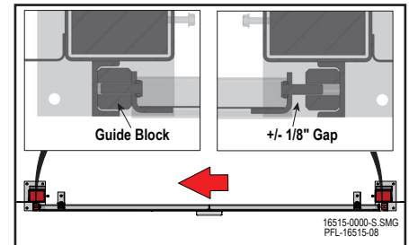
Guide Block Gap Figure 16-61
