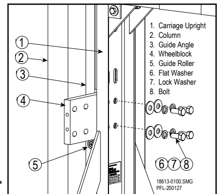
Upper Wheelblock Placement Figure 12-21
