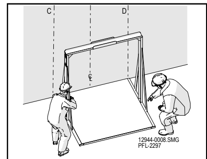
Place Carriage Figure 11-7
