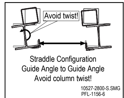
Avoid Twist Figure 12-32
