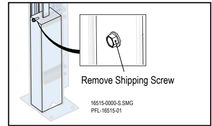
Post Assembly Counterweight Figure 16-33
