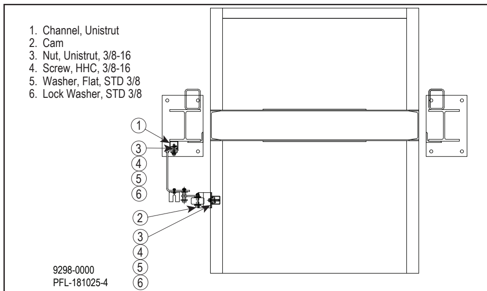
Straddle Placement Figure 17-11
