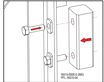
Attach Guide Blocks to the Gate Panel Figure 16-70
