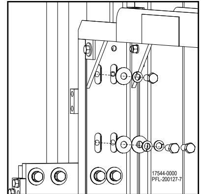
Insert Hex Head Screws Figure 12-28
