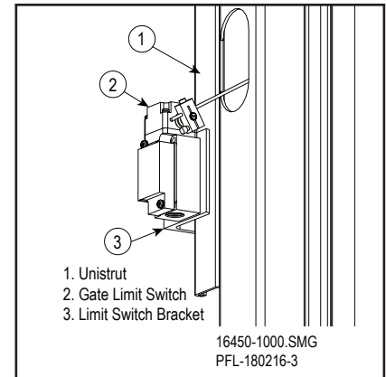
Attach Gate Limit Switch Figure 16-80
