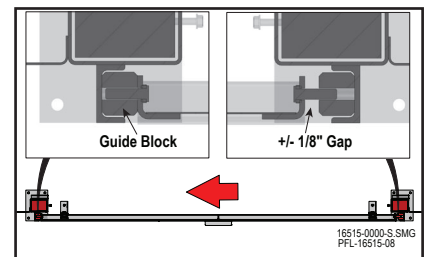
Guide Block Gap Figure 16-76
