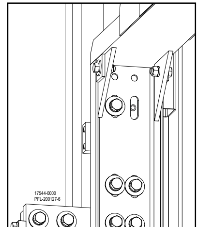
Attach Safety Cam Figure 12-29
