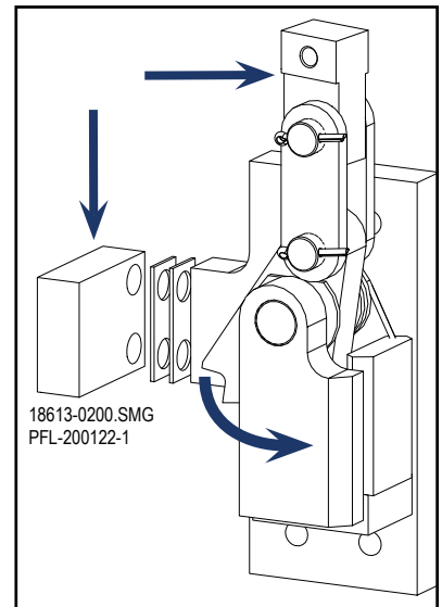
Remove Safety Cam Shoe and Rotate the Safety Cam Figure 12-25
