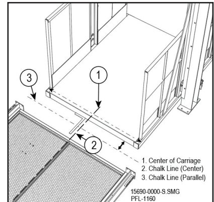
Establish Center and Parallel Line Figure 16-13
