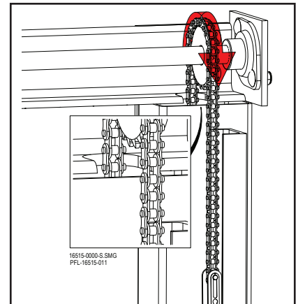
Thread Chain Over the Sprockets Figure 16-53
