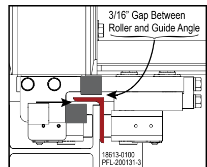
Verify Gap Figure 12-33
