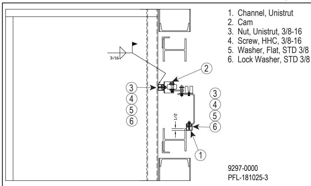
Cantilever Placement Figure 17-12
