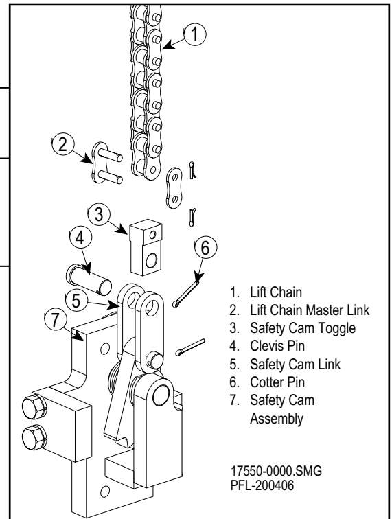
Attach the Lift Chain to the Wheelblock Figure 12-41
