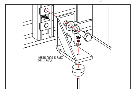
Attach Panel Bumper Figure 16-57
