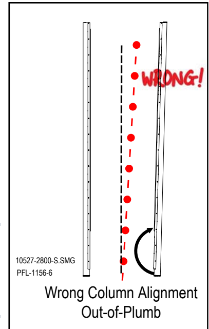
Column Alignment Out-of-Plumb Figure 12-31
