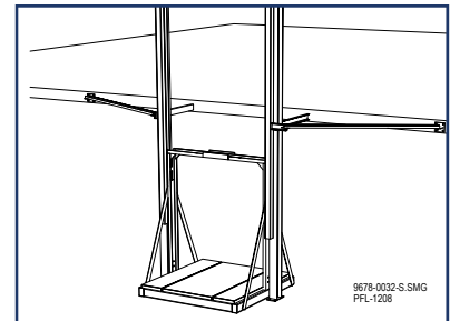
Tack Weld Bracing Figure 12-36
