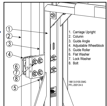
Attach Adjustable Wheelblock Figure 12-22
