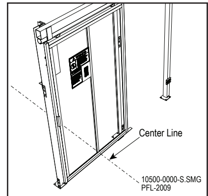
Align the Raised Gate Assembly Figure 16-6
