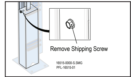
Post Assembly Counterweight Figure 16-64
