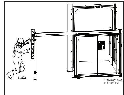
Plumb the Gate Figure 16-7
