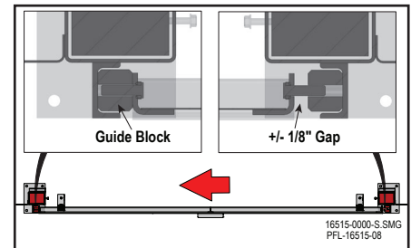
Guide Block Gap Figure 16-48
