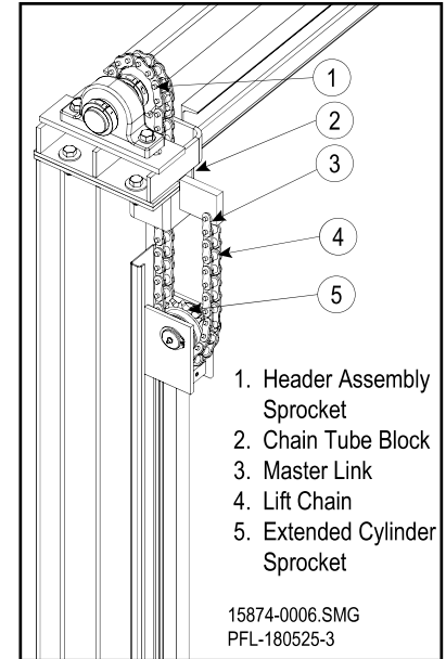
Drop the Lift Chain Down the Chain Tube Block Figure 12-40
